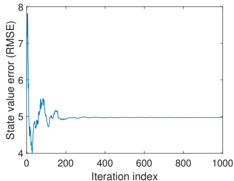
(e) The value error does not converge to zero.
