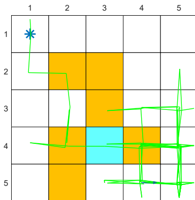
(b) An episode with 100 steps.
