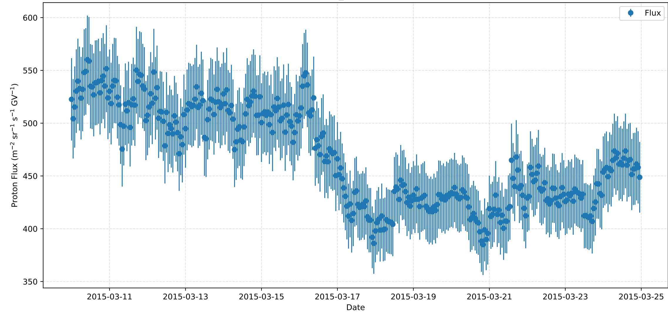
Flux \pm error_bar [1.0-1.16] GV
