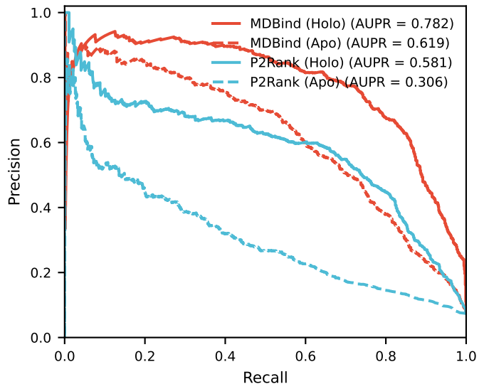
Precision-Recall Curve
