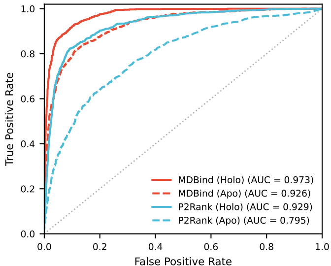
ROC Curve
