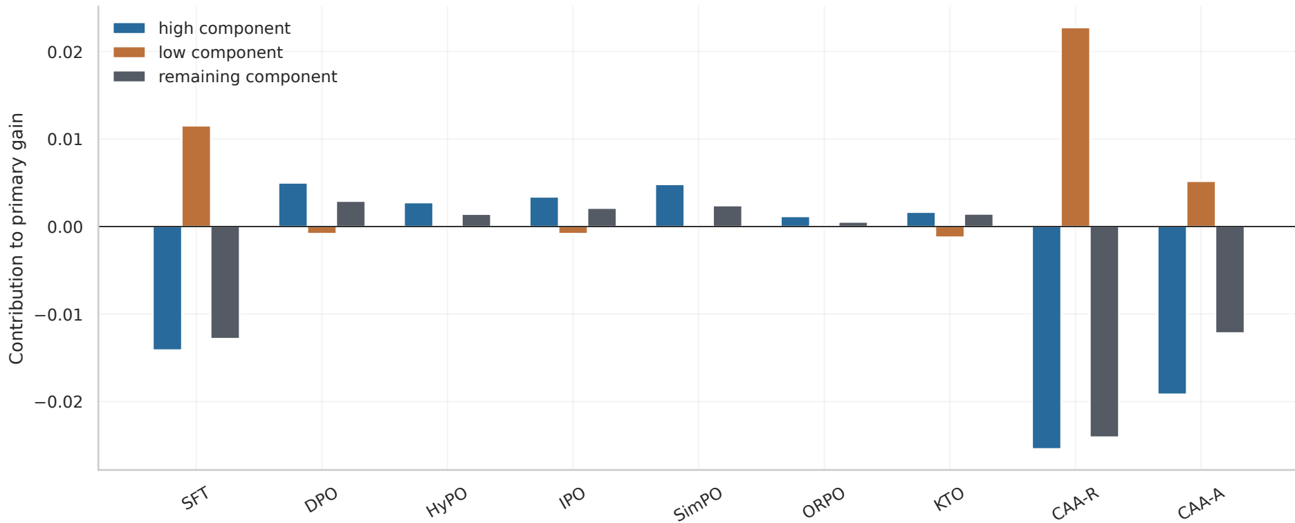
Components of the AITA probability shift
