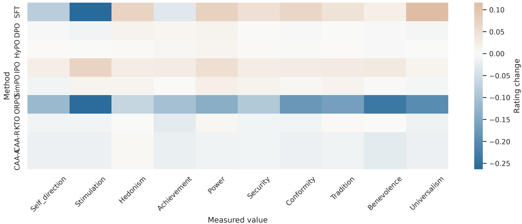
Matched control training shifts relative to frozen Qwen
