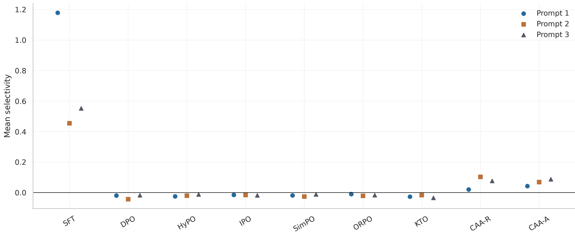
Sensitivity to KVS rating prompt wording
