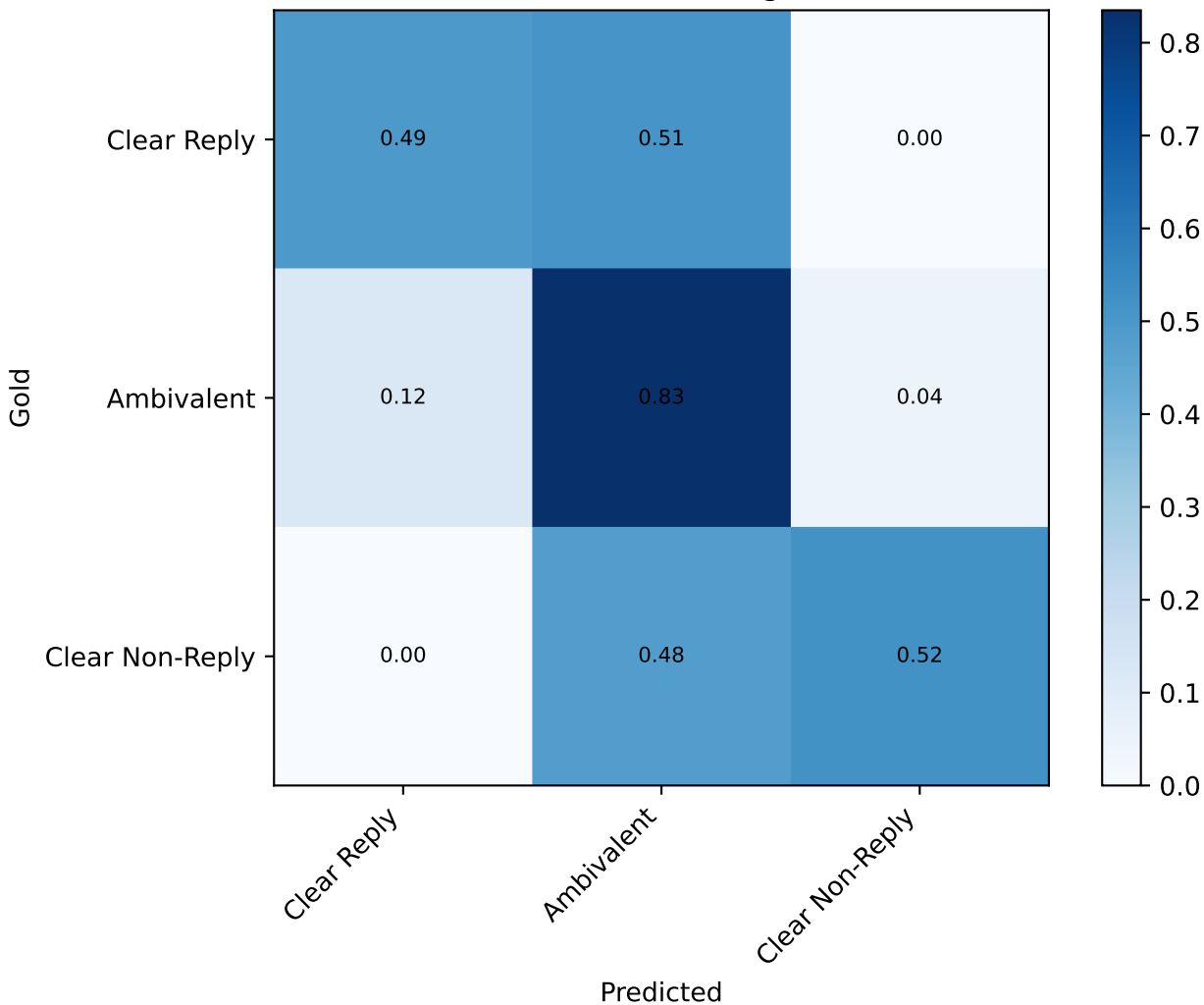
TASK1 confusion matrix (normalized) DeBERTa-v3-large
