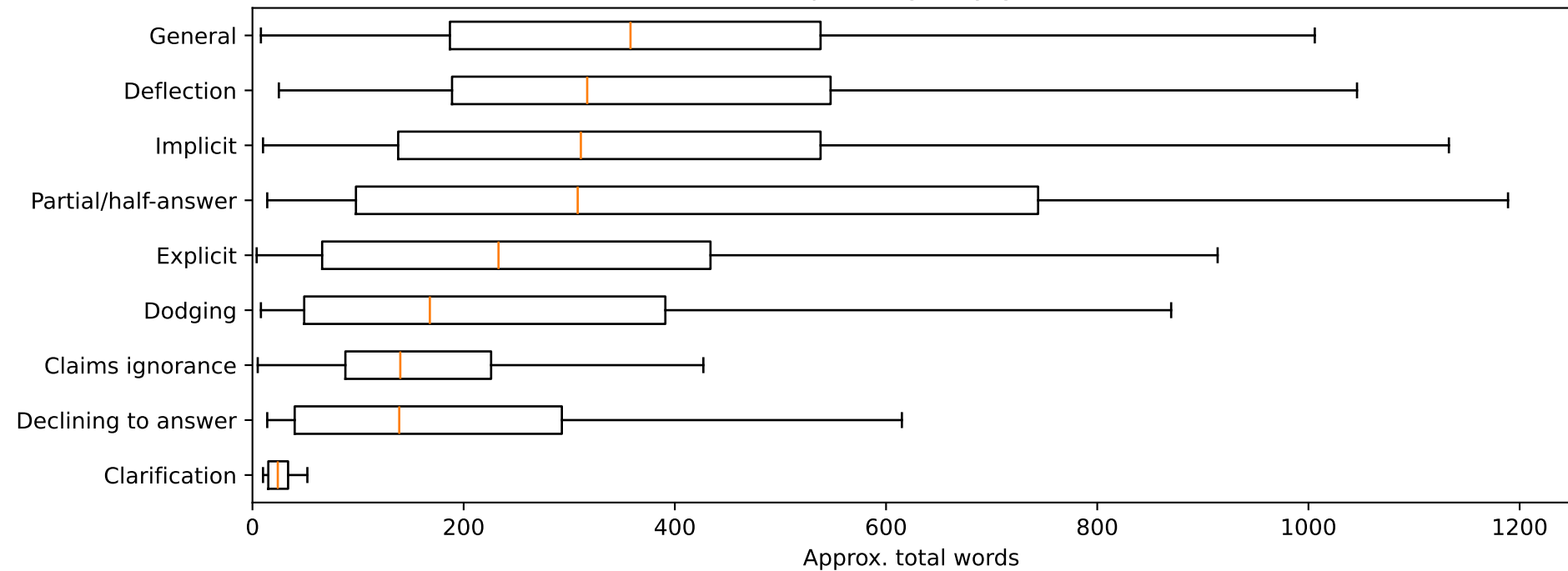
TASK2 input length by gold label
