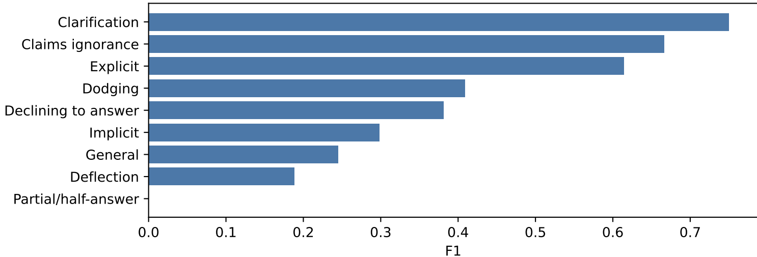
TASK2 per-class F1: DeBERTa-xlarge
