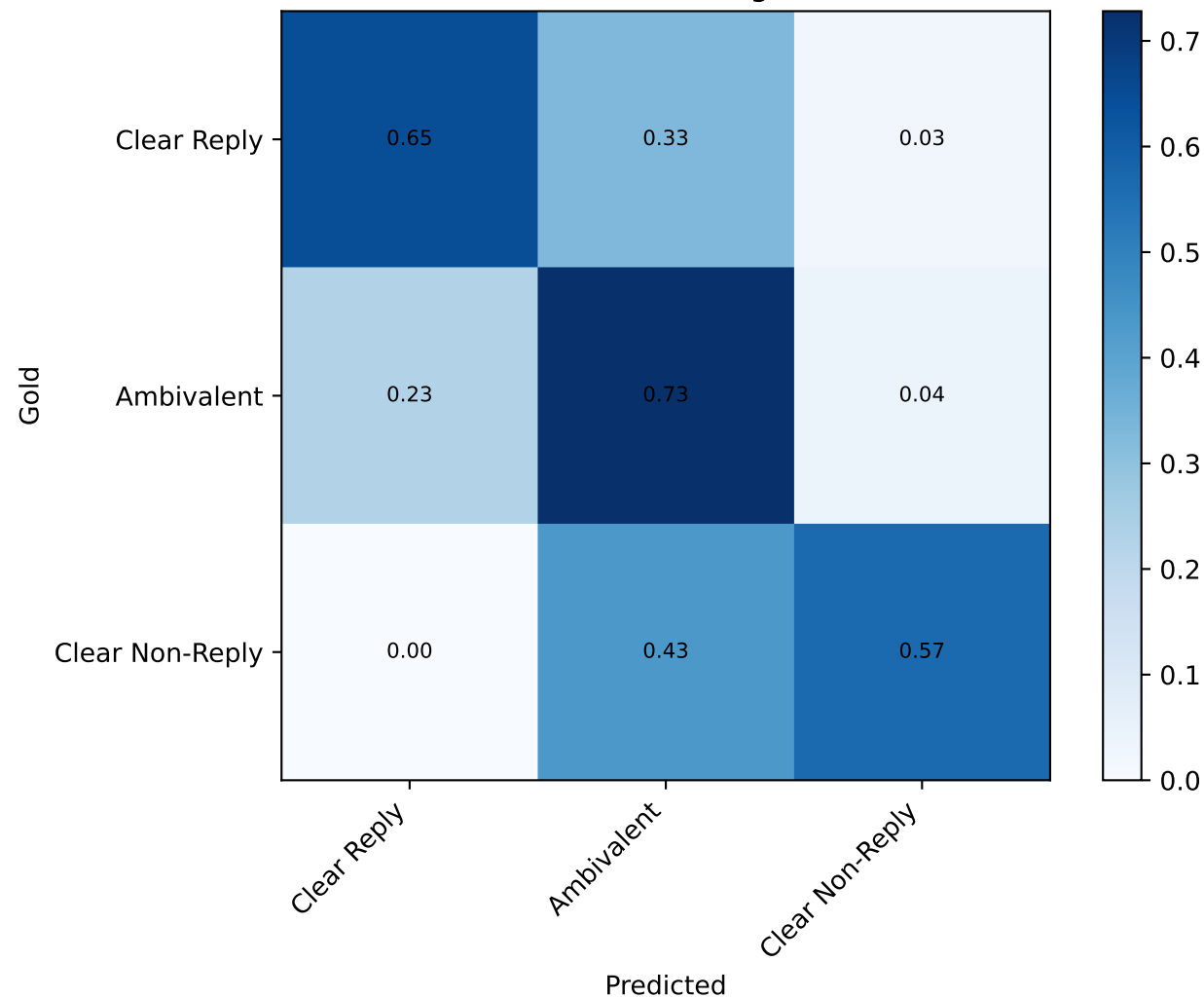
TASK1 confusion matrix (normalized)
