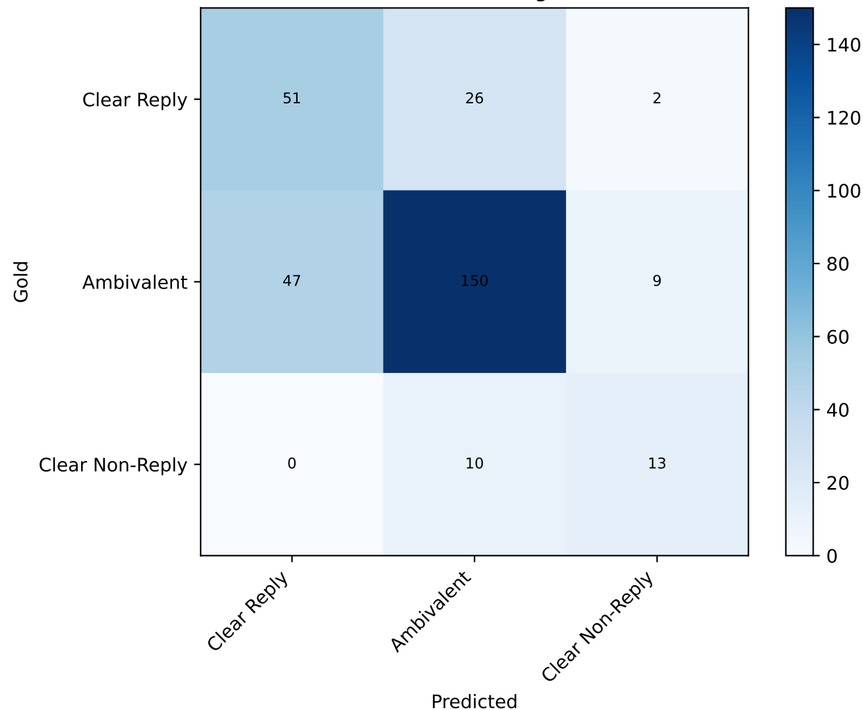
TASK1 confusion matrix (raw) DeBERTa-xlarge
