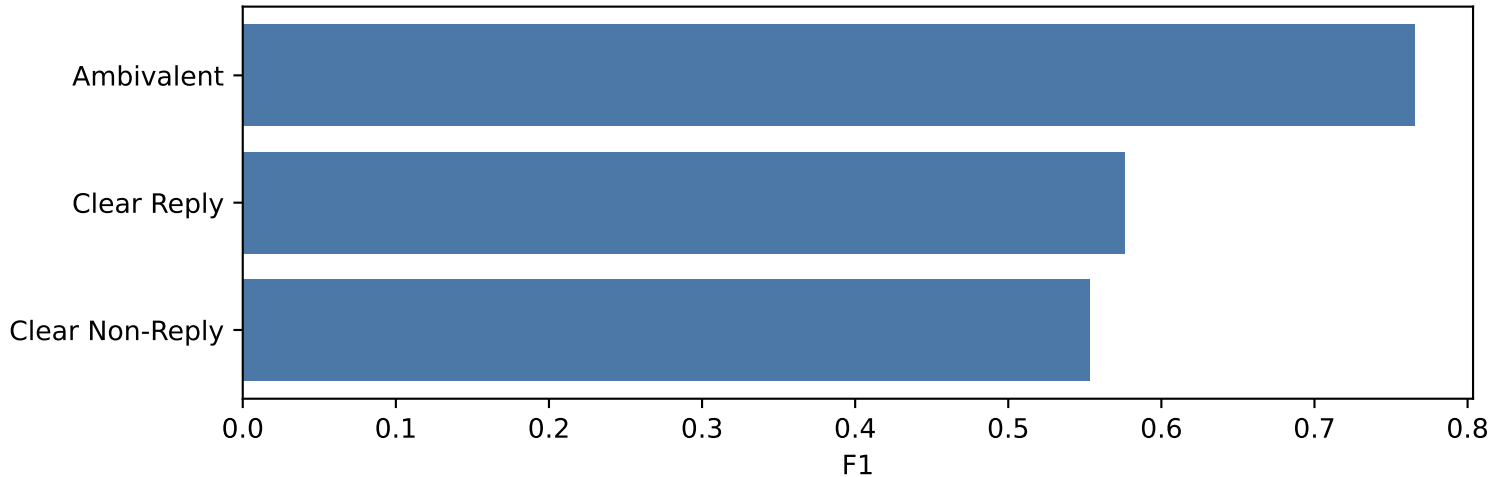
TASK1 per-class F1: DeBERTa-xlarge
