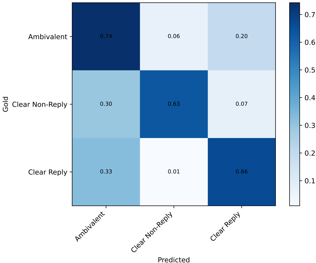
TASK2 confusion matrix (normalized) deberta-v3-base multi-task
