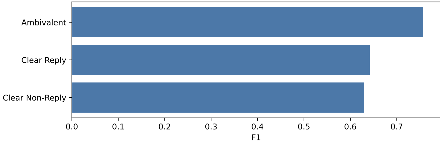
TASK2 per-class F1: DeBERTa-v3-base multi-task
