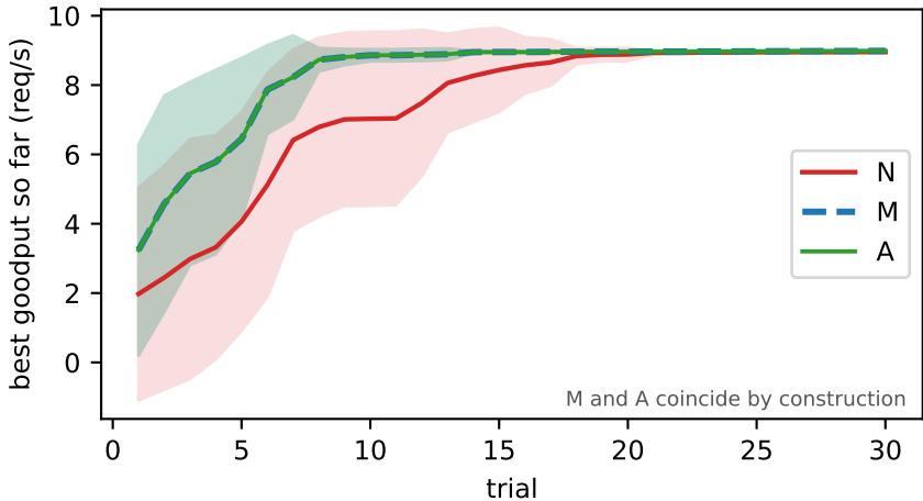
Best-so-far goodput (20 seeds, mean \pm std)
