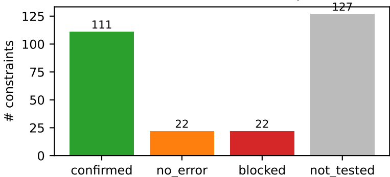
Execution-based falsification status (vLLM v0.30.0)
