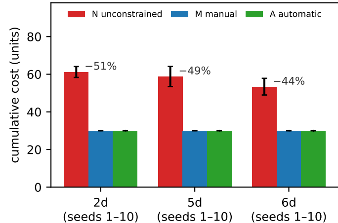
(a) Dimension scaling (qps = 12)
