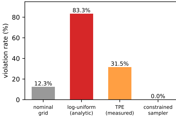
(a) Waste depends on the sampling distribution
