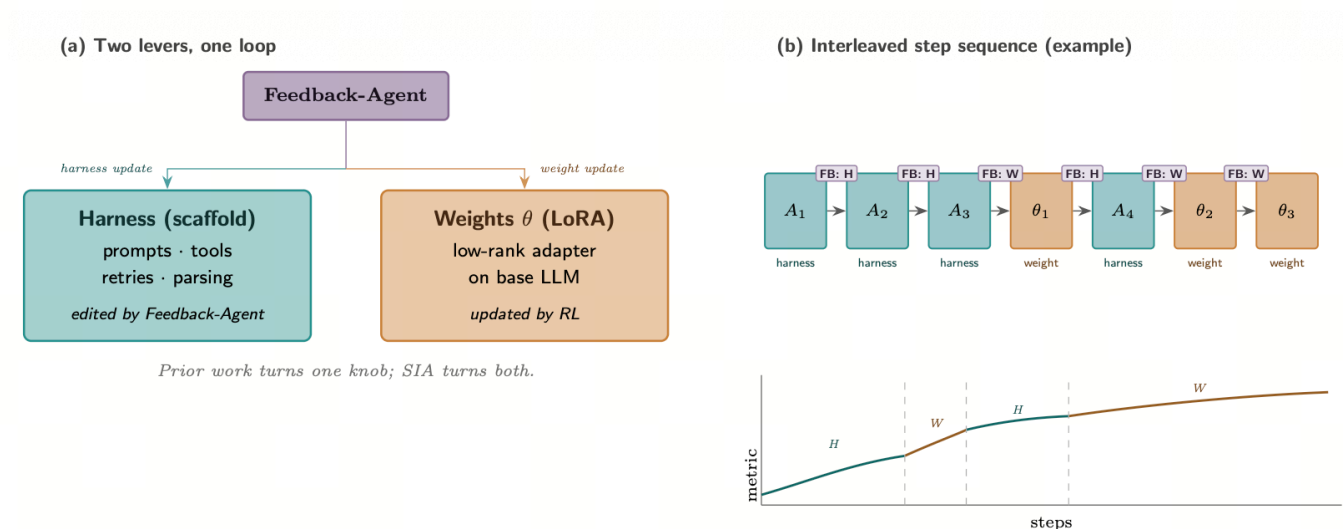
Figure 17: The Feedback-Agent in SIA decides the next iteration type.
