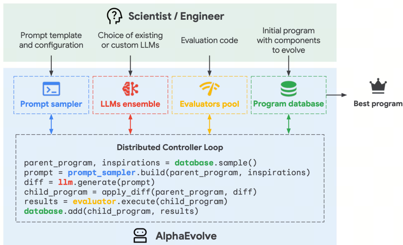
Figure 15: How AlphaEvolve works. (Image source: Novikov et al. 2025 )
