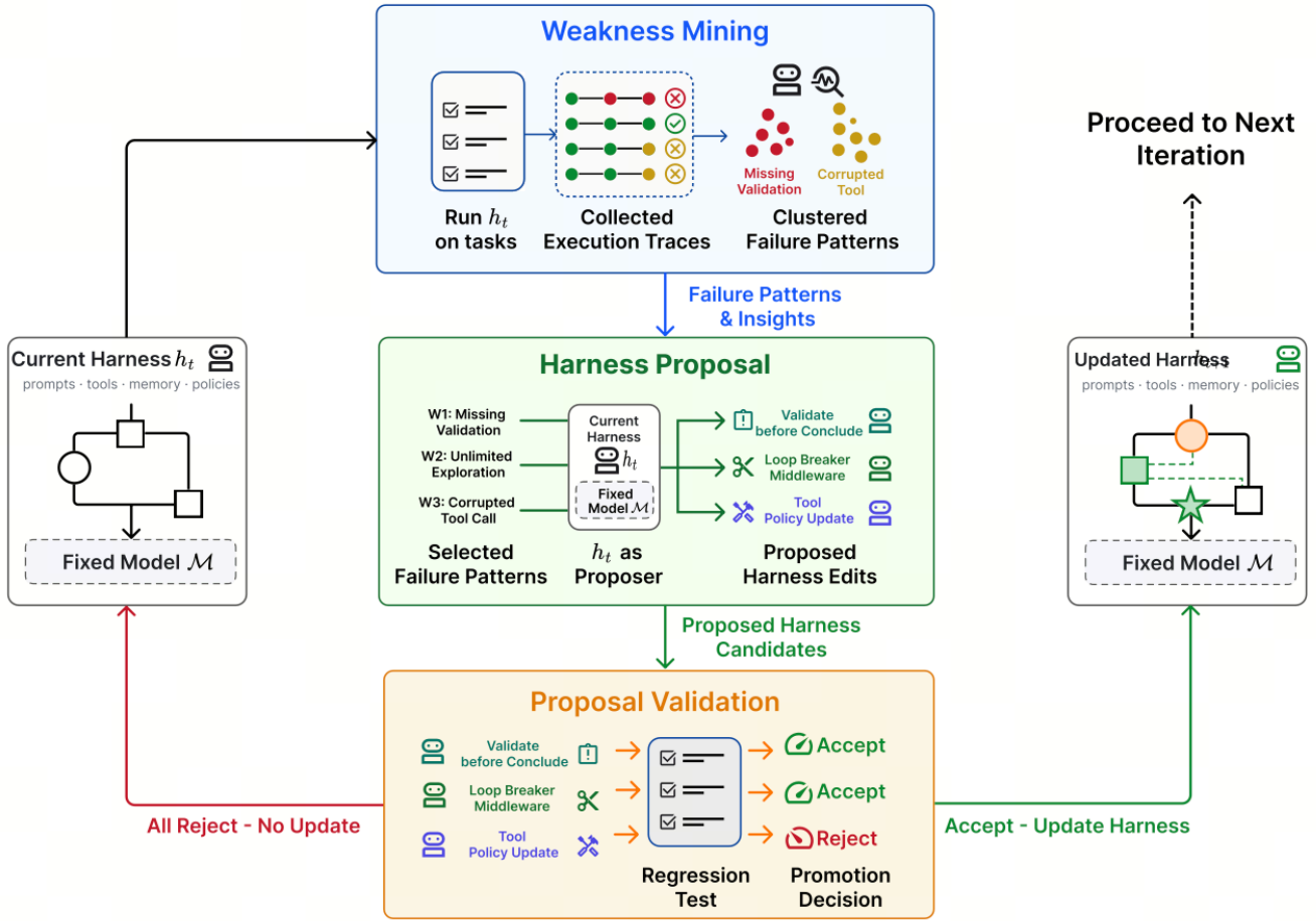
Figure 14: Self-Harness uses a loop of weakness mining, bounded harness proposal, and validation to update a harness. (Image source: Zhang et al. 2026 )
