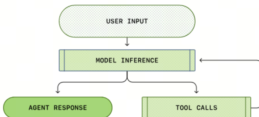
Figure 1: A simplified Codex agent loop: the agent calls tools and tool responses affect the model's next generation.
