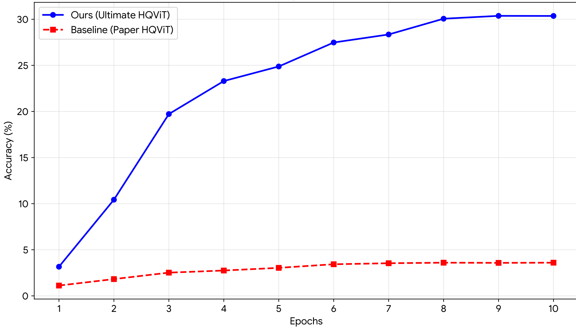
CIFAR-100 Training Accuracy Comparison
