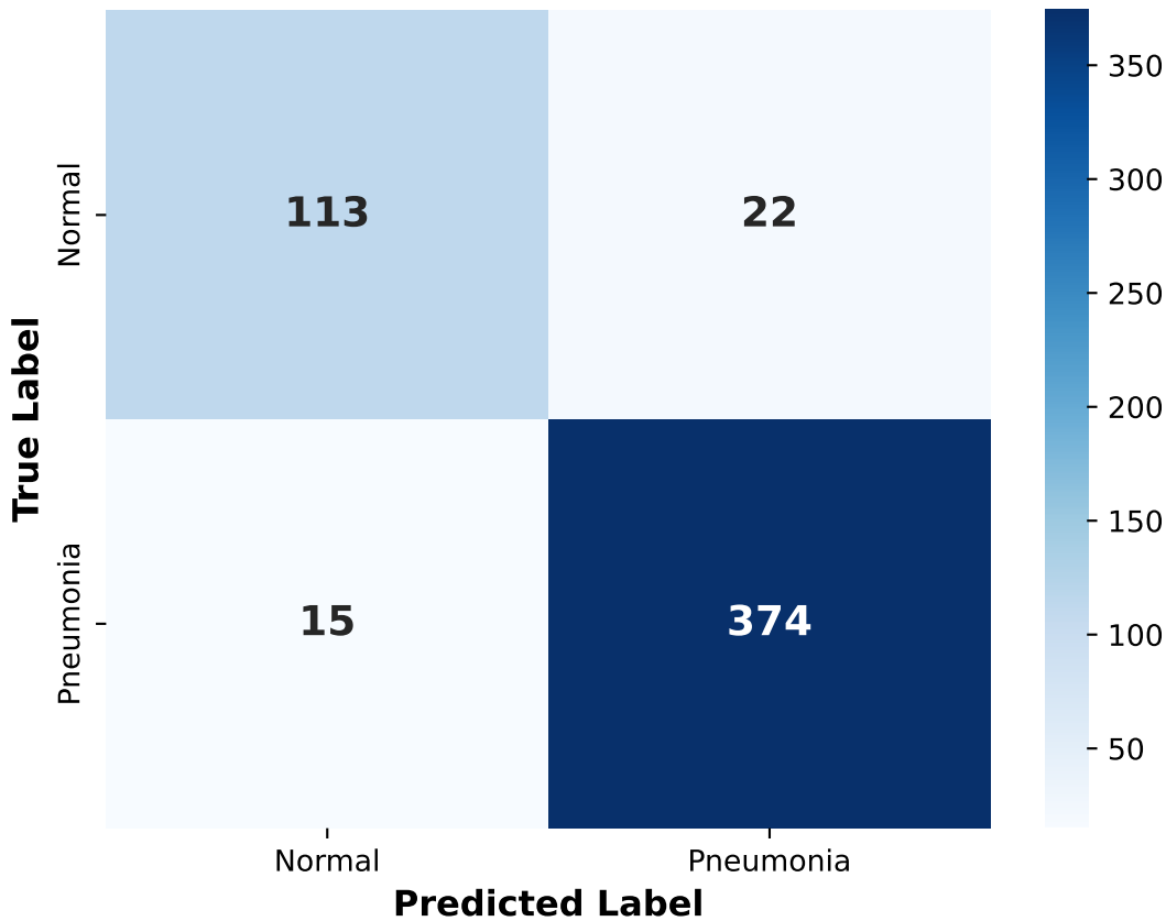
Confusion Matrix (HQViT + VQC + Focal)
