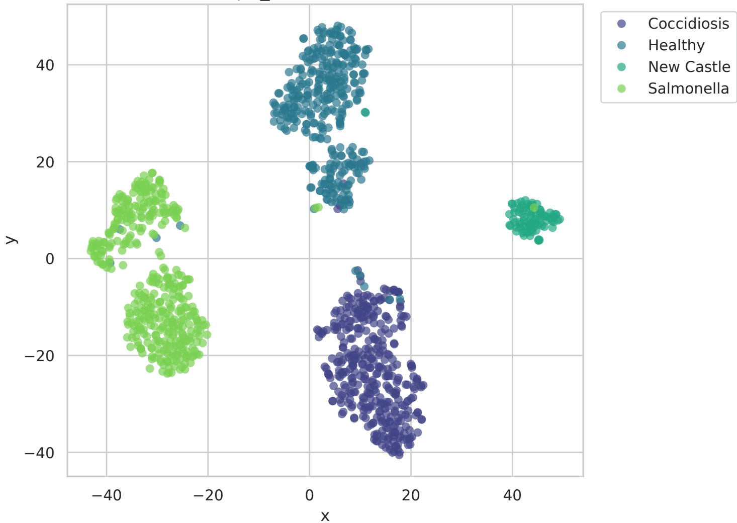
Exp3_Formatted - t-SNE
