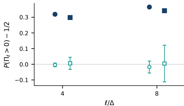
b Instantaneous forward bias
