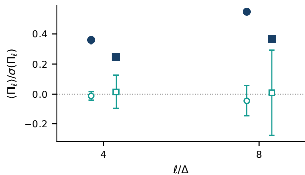
a Mean transfer
