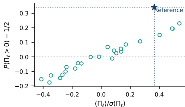
d Independent scale 8: mean vs sign
