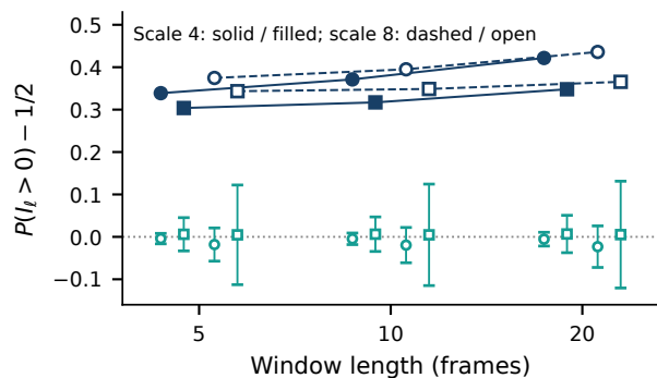
c Finite-window bias
