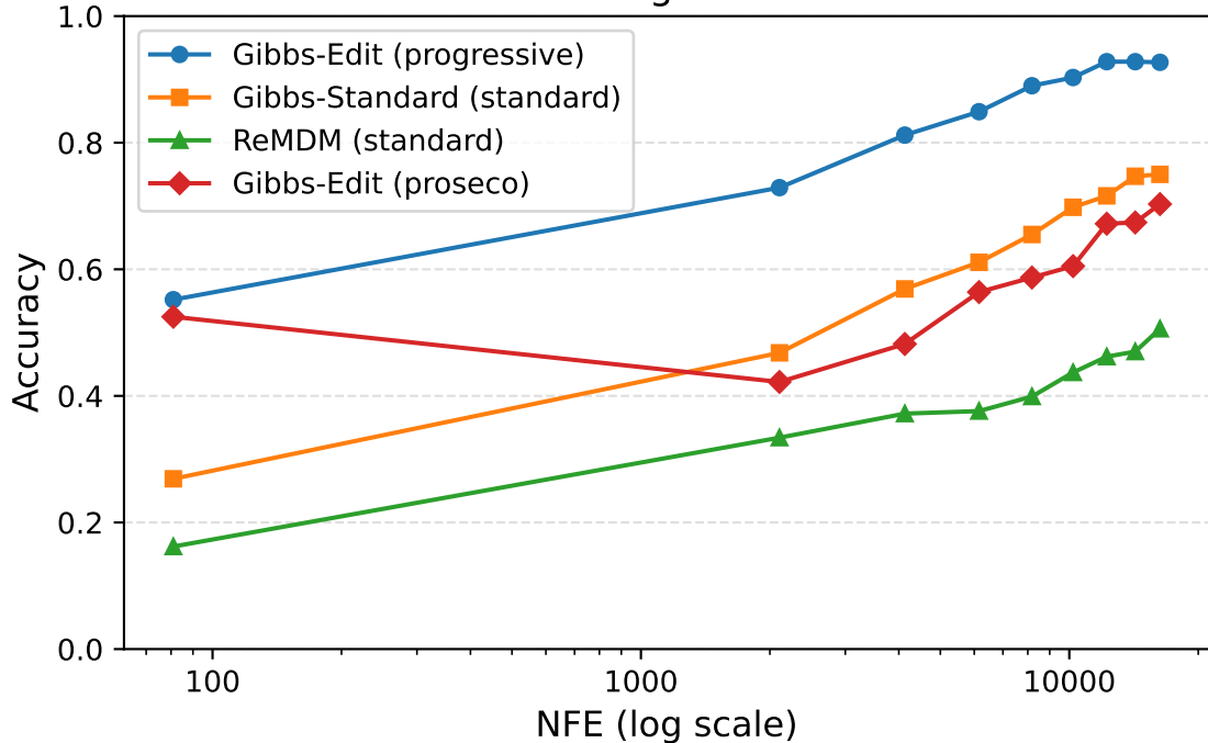
Inference Scaling on Hard Sudoku
