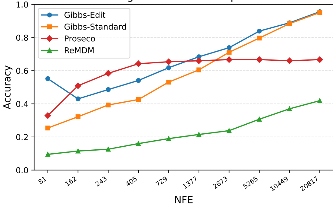
Progressive-Edit Checkpoint
