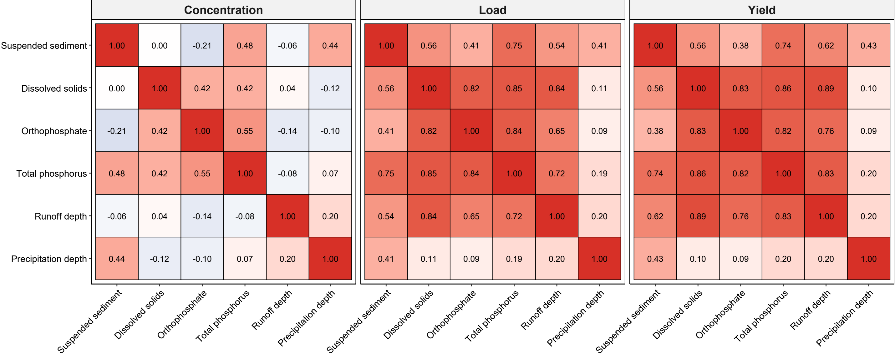
Correlations among water-quality and hydrologic variables
