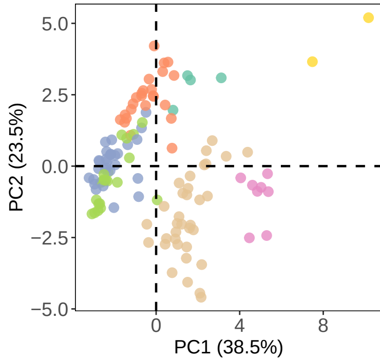
K-means Clusters in PCA Space
