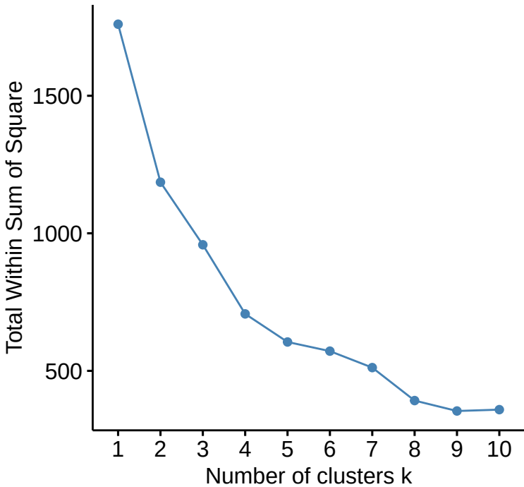
Elbow Method for k-means
