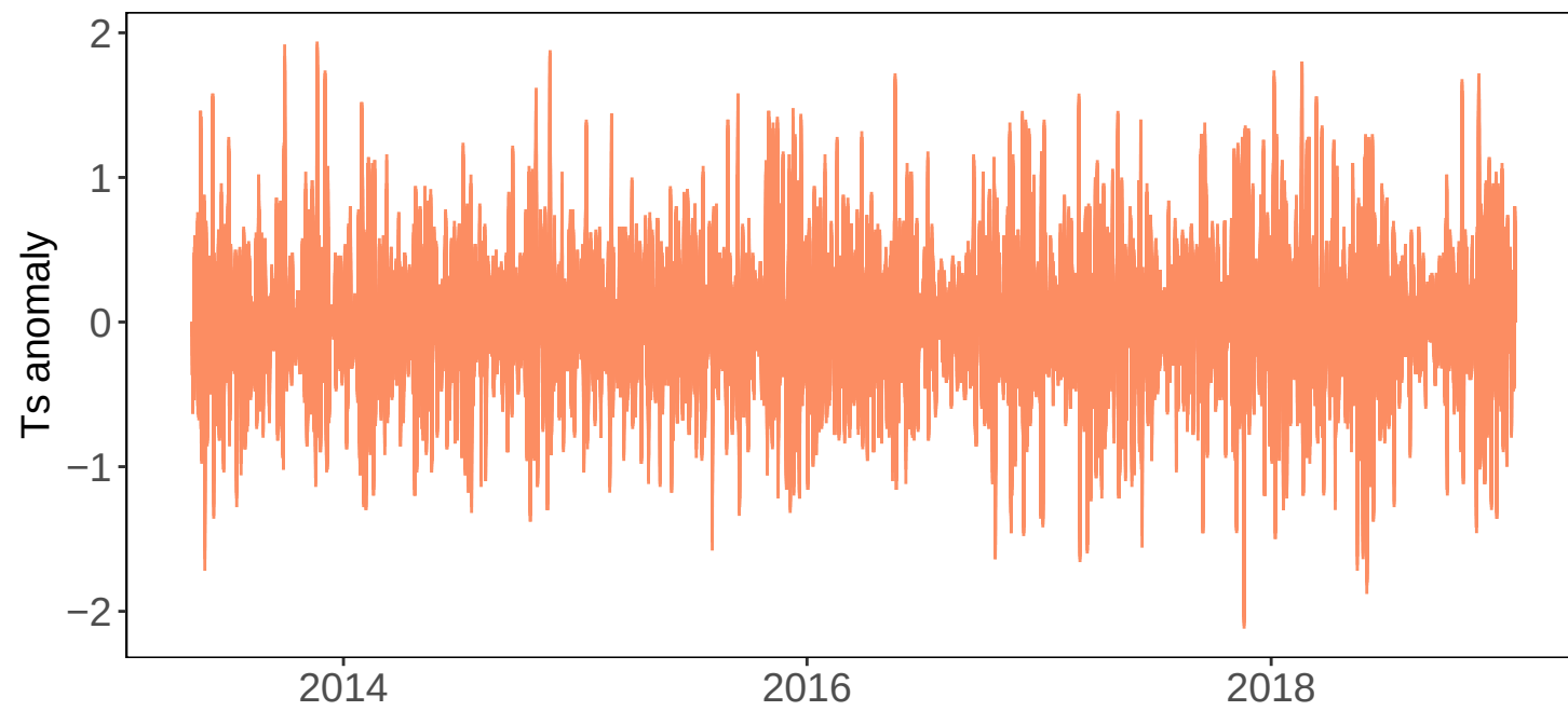
Ts anomaly
