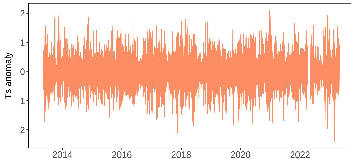
Ts anomaly
