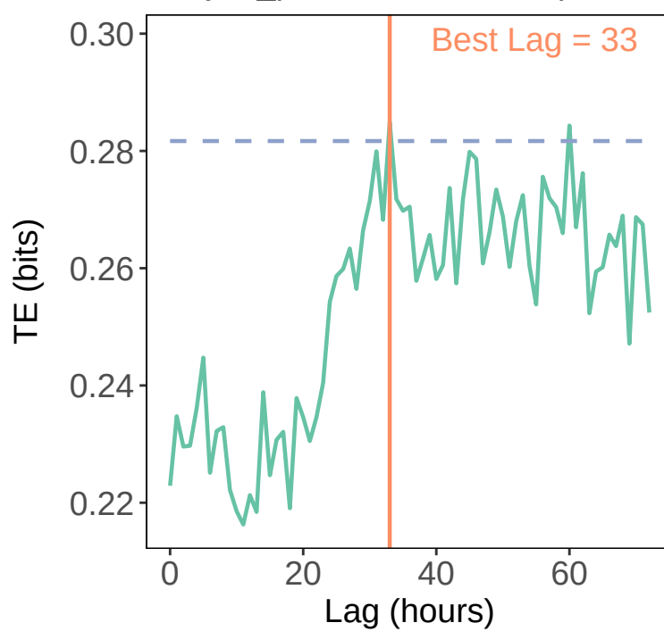
Desync_post climate -&gt; response
