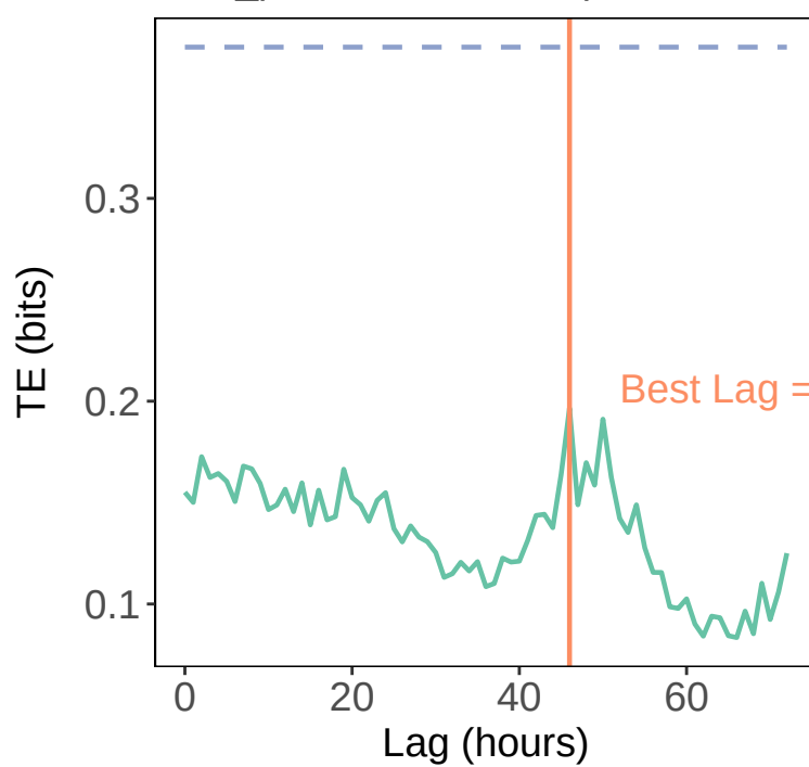
Shift_pre climate -&gt; response
