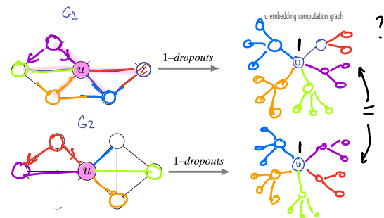
Figure 3: Example of two graphs not separable by 1-dropouts (left side). In both of the graphs, for any of the 1-dropouts, u observes the same tree structure for d=2 , shown on the right side.
