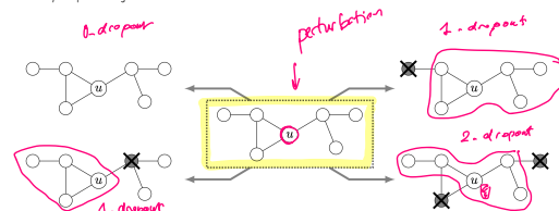
Figure 1: Illustration of 4 possible dropout combinations from an example 2-hop neighborhood around u : a 0-dropout, two different 1-dropouts and a 2-dropout. (DropGNN Papp et al., 2021)
