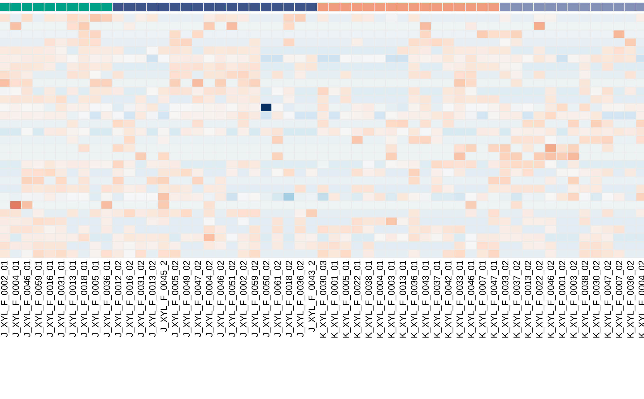
Top 30 variable features (z-scored)
