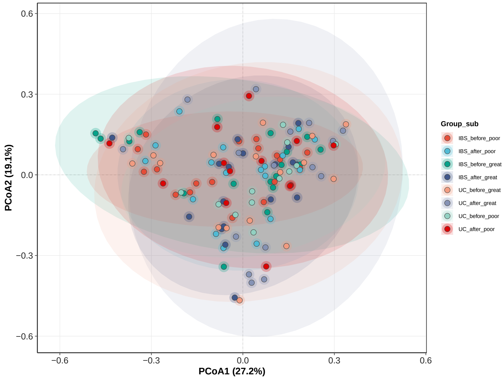
PCoA (Bray-Curtis beta diversity)
