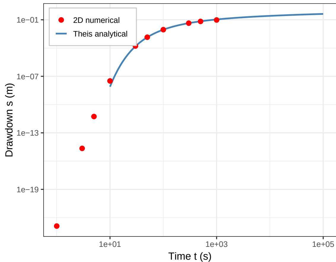
(b) Log-log drawdown curve
