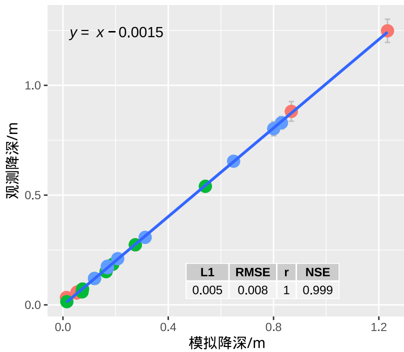
(c) 3次抽水试验
