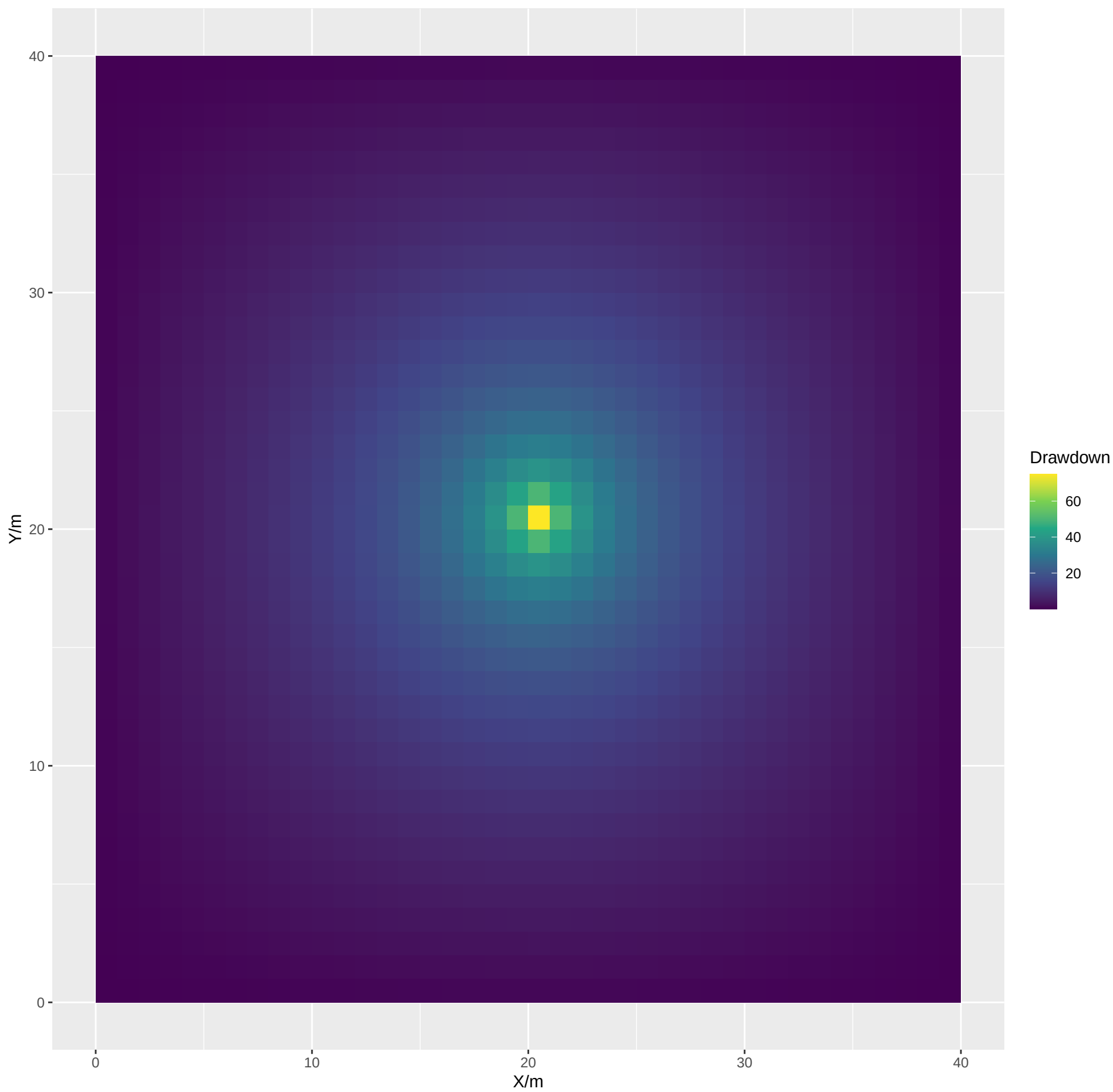
2D Steady-State Drawdown Distribution
