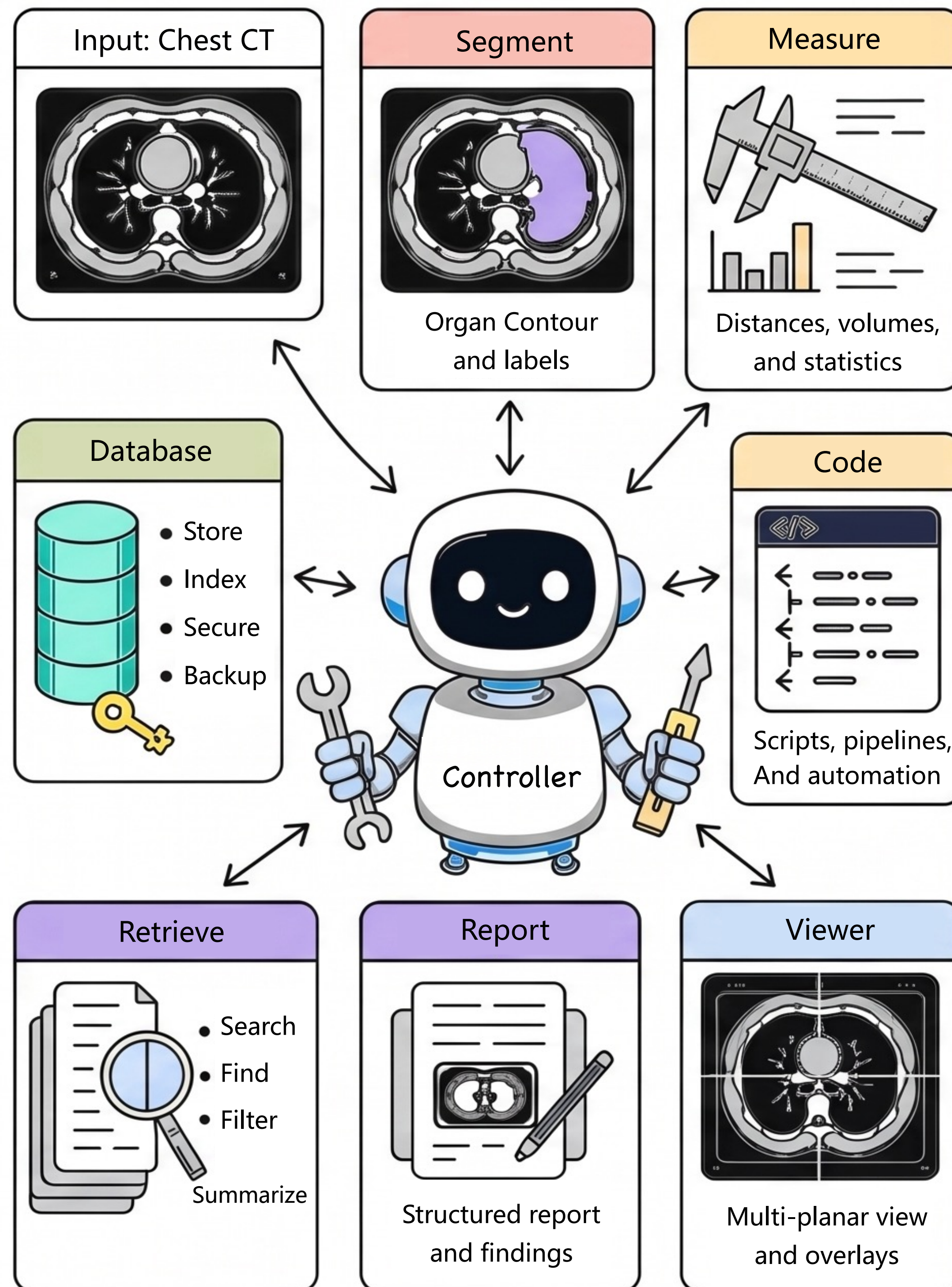
(a) Single Agent Tool-Augmented
