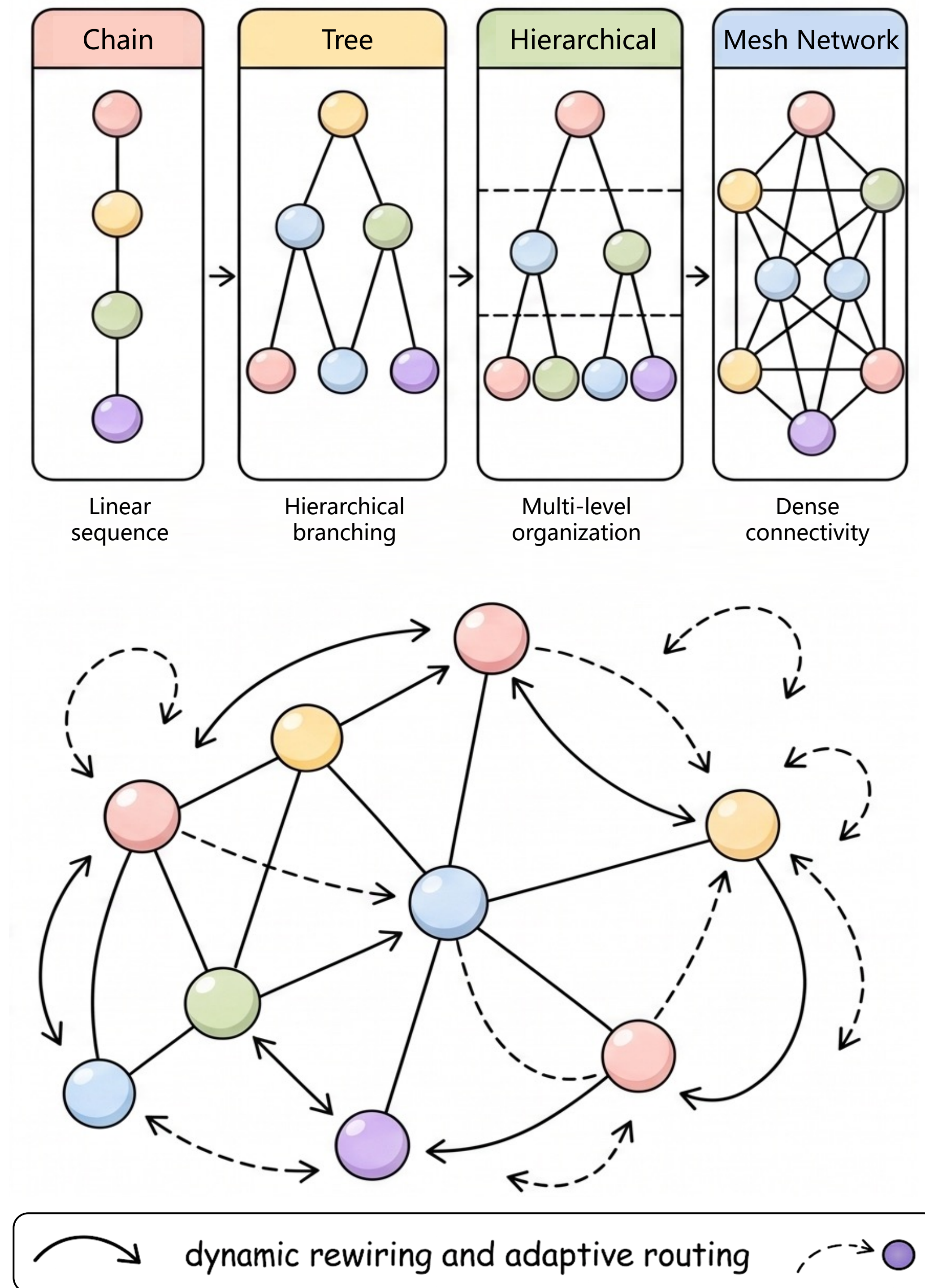
(c) Orchestration Topologies
