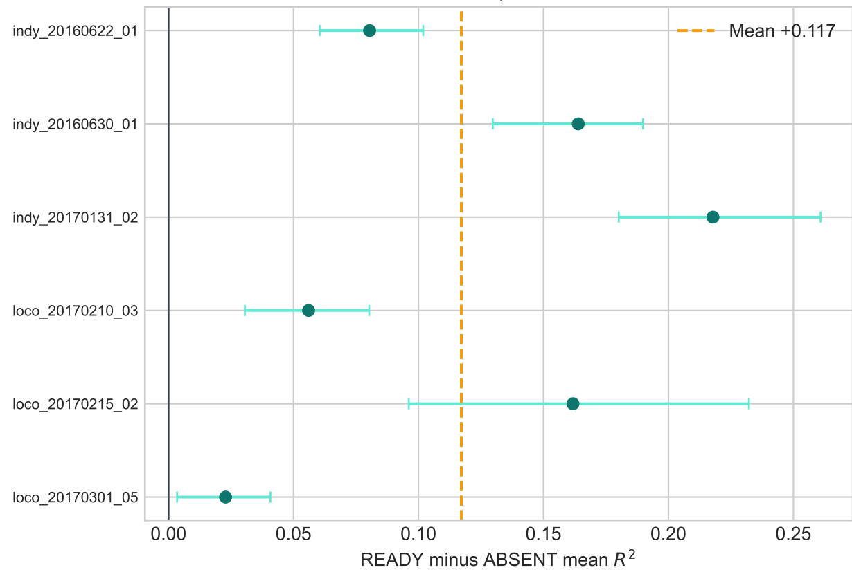
Reach-bootstrap 95% intervals
