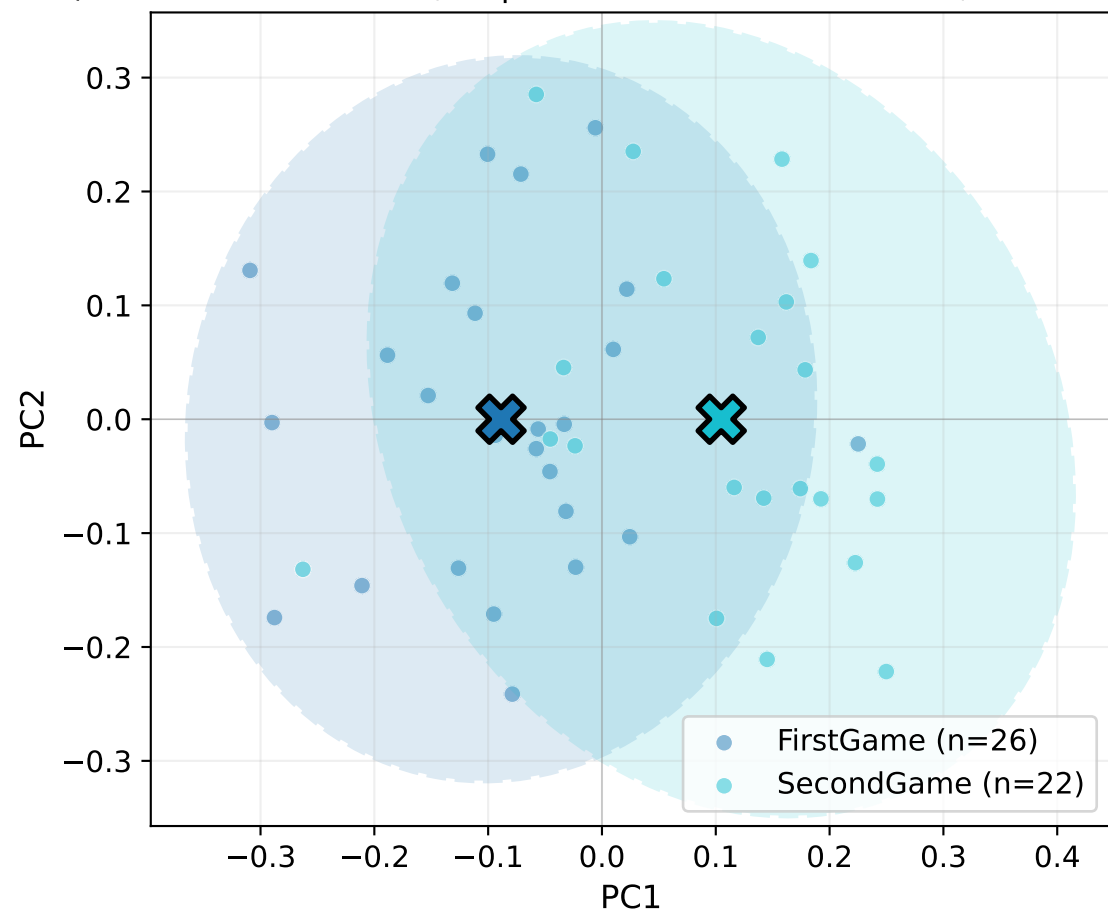
ENA Space: Reproducibility Visualization (dots = individual runs, ellipses = 95% confidence area, X = centroid)
