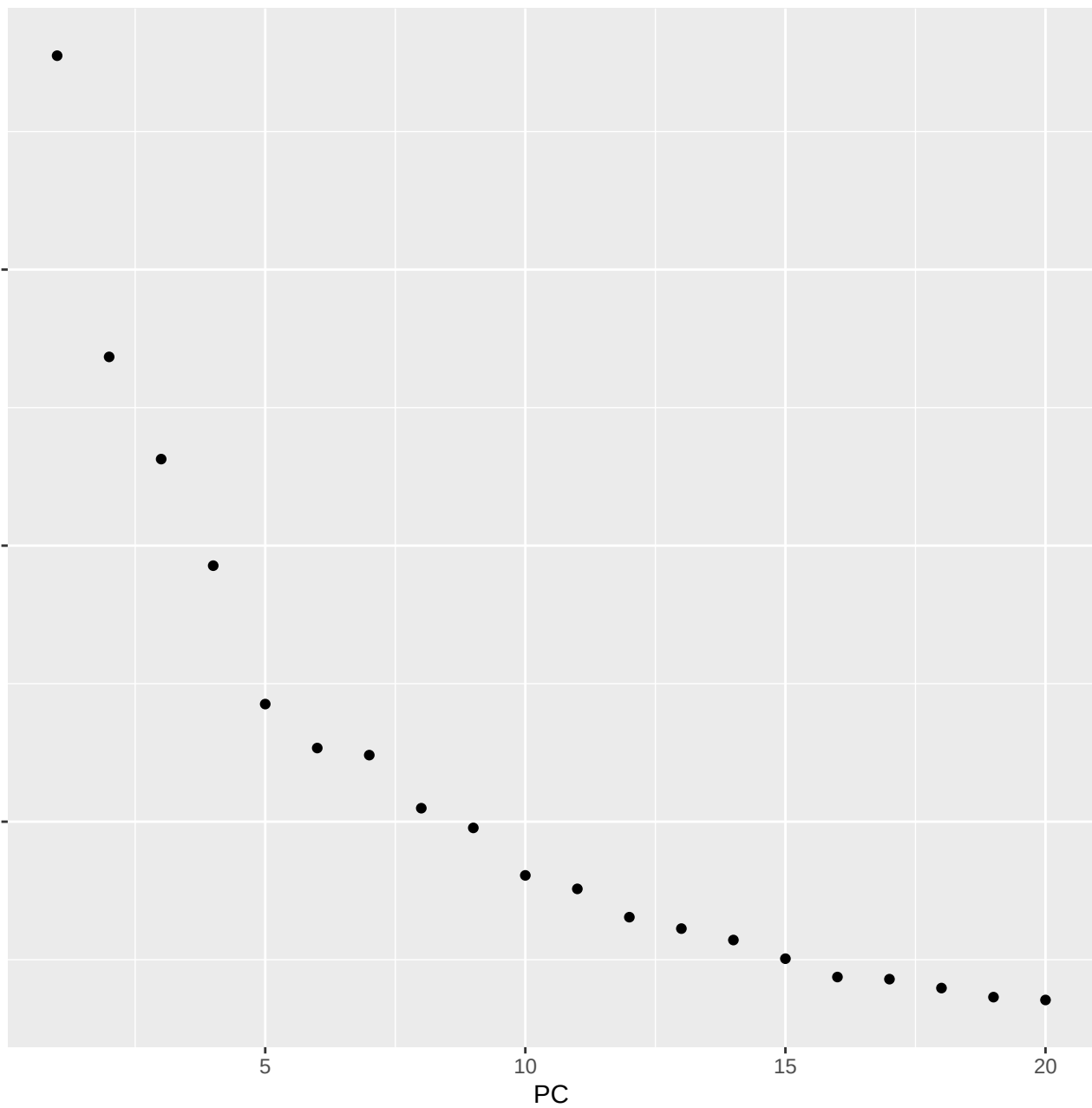
Standard Deviation of PC
