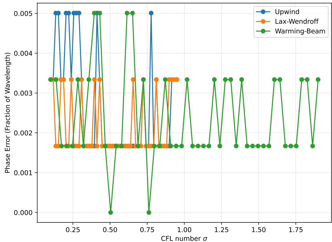
Phase Error vs. CFL Number
