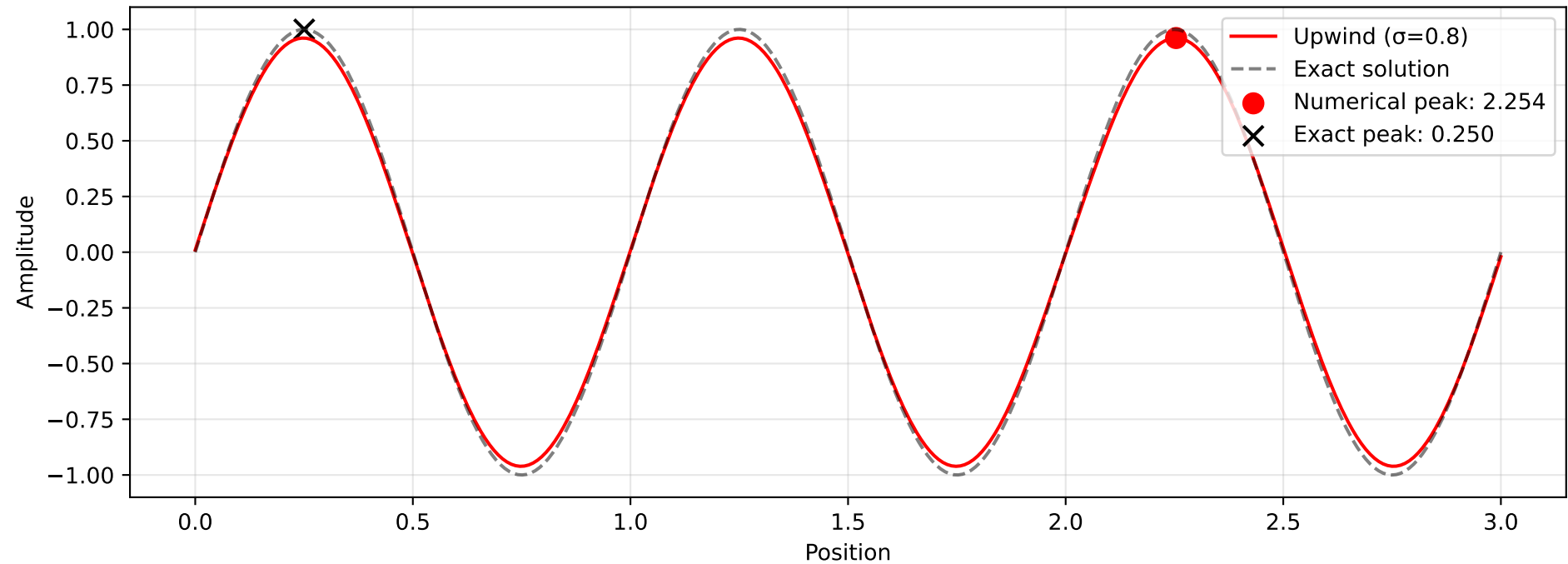
Dissipation and Dispersion Analysis - Upwind
