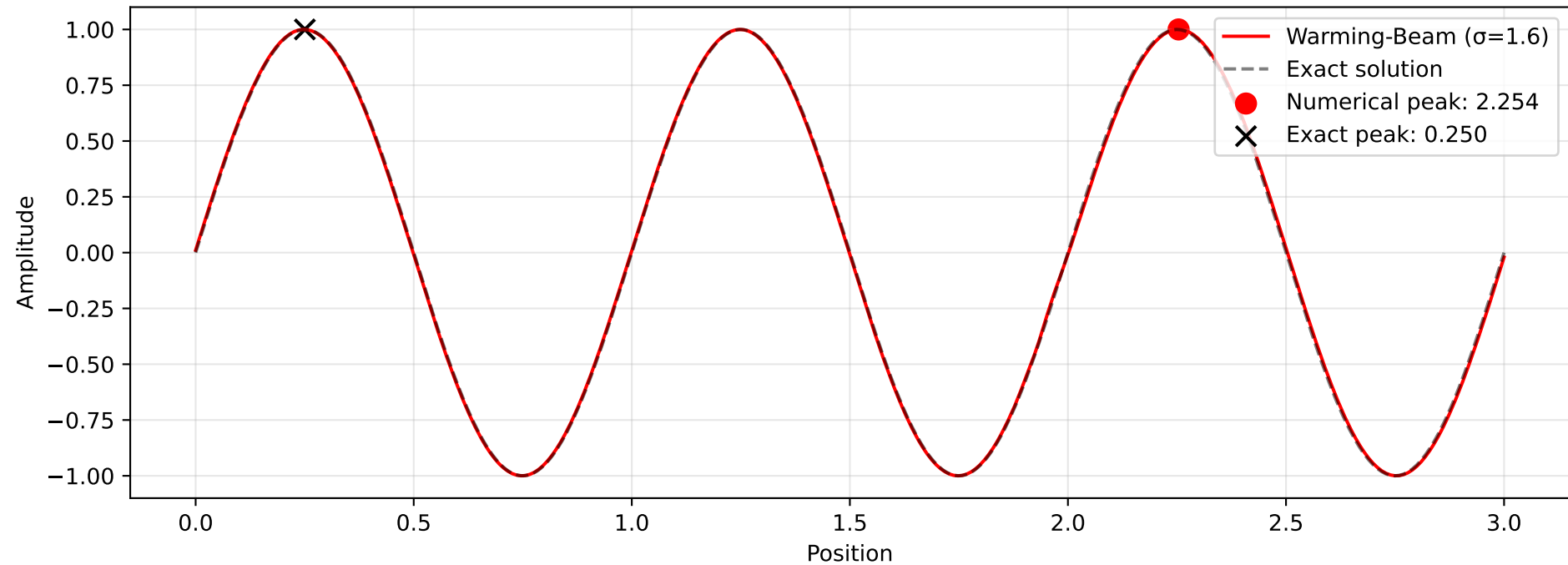
Dissipation and Dispersion Analysis - Warming-Beam
