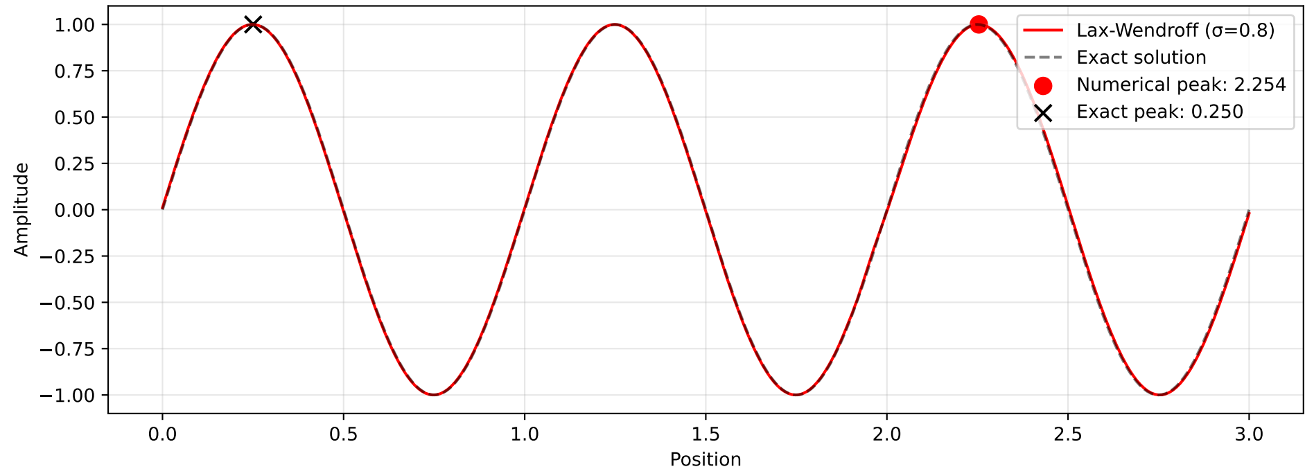
Dissipation and Dispersion Analysis - Lax-Wendroff
