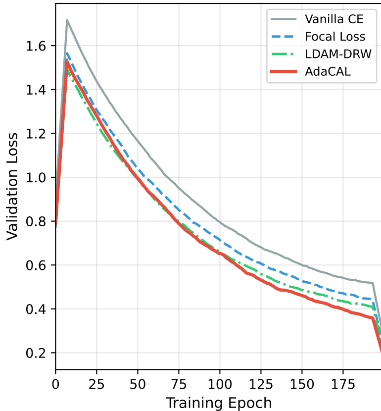
Validation Loss Convergence (LSTM, MIT-BIH Arrhythmia)
