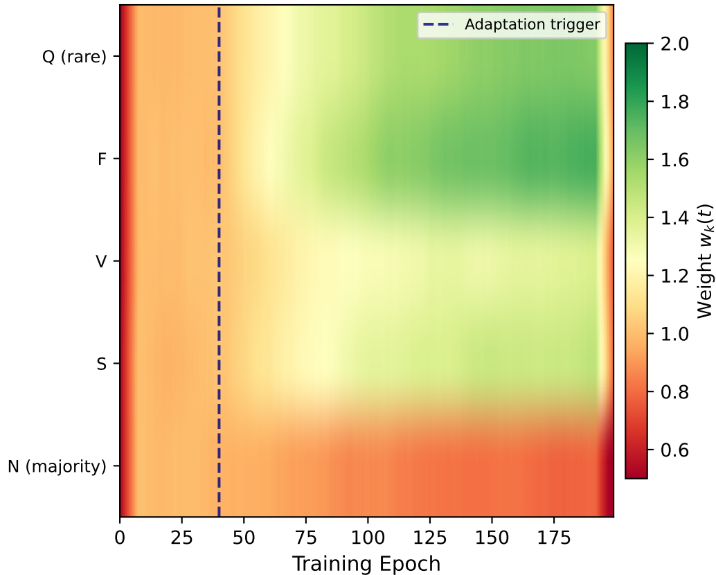
AdaCAL Adaptive Weight Trajectory w_k(t) per Class over Training
