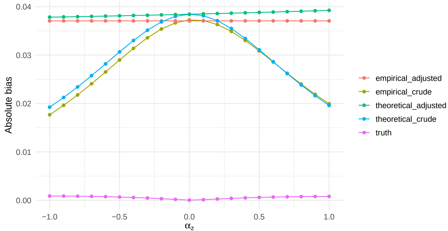
Bias under different \alpha_z values
