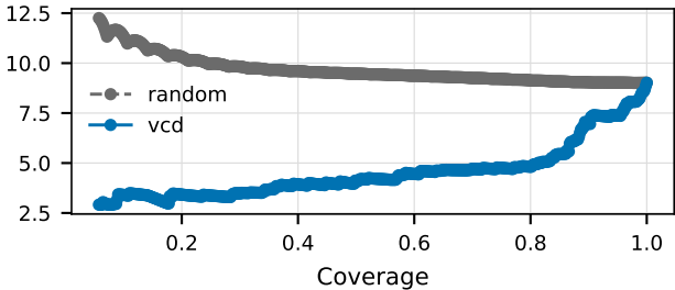
VCD risk-coverage
