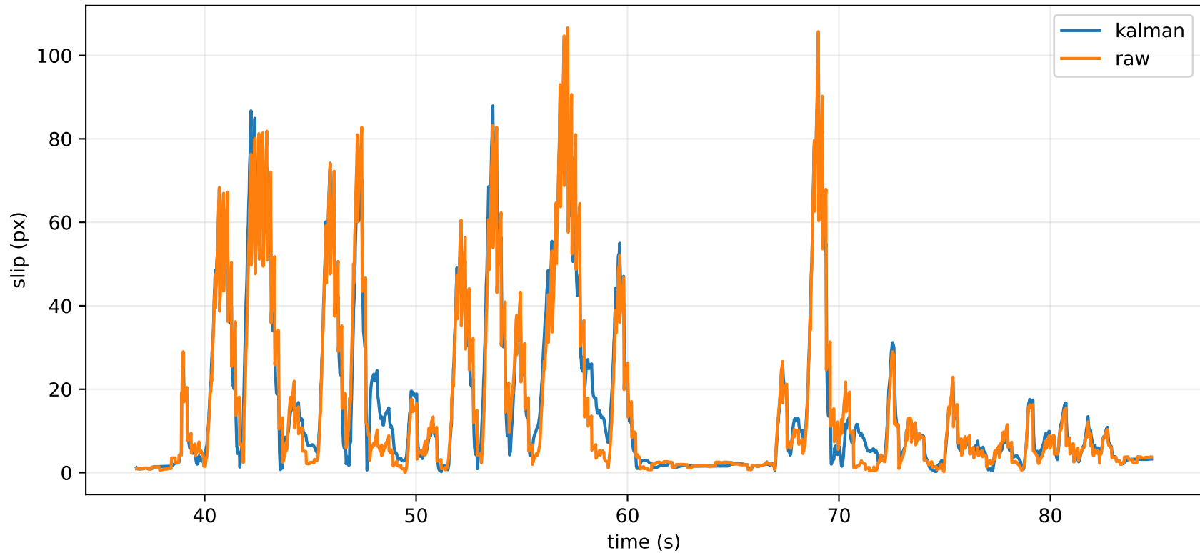
Screen-Space Slip
