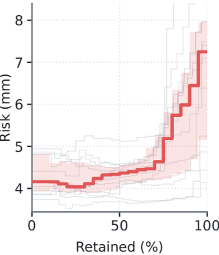
(c) VCD risk-coverage
